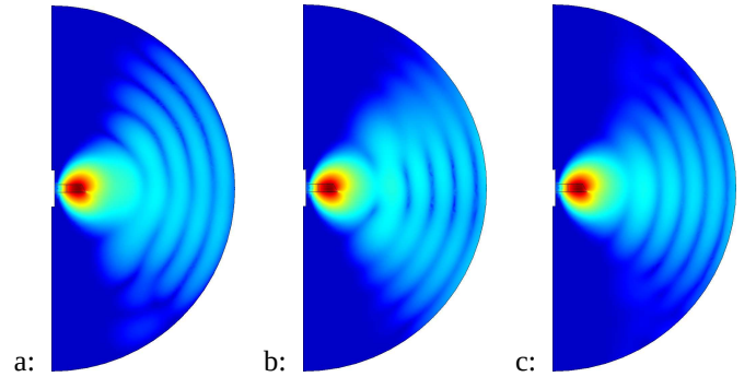
Fig. 5. Radiation associated with the same [\text{TE}_{p=1,m=11}, \lambda = 1263.6 \text{ nm}] whispering-gallery mode as presented in Fig. 4 (all three maps use the same absolute false-color scale): (a) standing-wave (equal outward- and inward-going) radiation with the outer semicircular boundary set as a magnetic wall; (b) the same but now with the boundary set as an electric wall; (c) somewhat traveling (more outward- than inward-going) radiation with the boundary's impedance set to that of an outward-going plane-wave in free space (and with the normal magnetic field constrained to vanish). That (c)'s radiation field is somewhat dimmer than (b)'s is consistent with the two different estimates of the resonator's radiative Q corresponding to (b) and (c) [see text].
