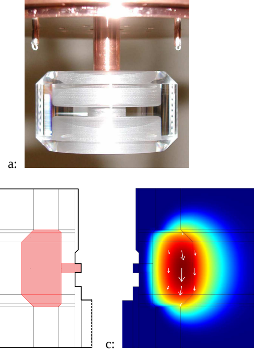
Fig. 7. (a) Close-up of NPL's cryo-sapphire resonator, with the main body of its outer copper can removed. The resonator's chamfered HEMEX sapphire ring has an outer diameter of \sim 46.0 mm and an axial height of \sim 25.1 mm. The ring's integral interior 'web', 3mm thick, lies parallel to, and is centered (axially) on, the ring's equatorial plane, and is supported through a central copper post. Optical refraction at the ring's outer surface falsely exaggerates its internal diameter. Above the ring are two loop probes for coupling electromagnetically to the resonator's operational whispering-gallery mode. (b) geometry of the resonator in medial cross-section; pink/grey indicates sapphire, white free space; bounding these dielectric domains, and shown as solid black lines, are copper surfaces belonging to the resonator's can and web-supporting post [the dashed vertical line (lower right) runs along the resonator's cylindrical axis ( r = 0 )]. (c) false-color map (logarithmic scale) of |\mathbf{H}|^2 for the resonator's 11th-azimuthal-mode-order fundamental quasi-transverse-magnetic ( N_{111} in ref. [7]'s notation) whispering-gallery mode at 9.146177 GHz (simulated), as detailed on the 6th row of TABLE II. The white arrows indicate the magnitude and direction of this mode's electric field strength ( \mathbf{E} ) in the medial plane.
