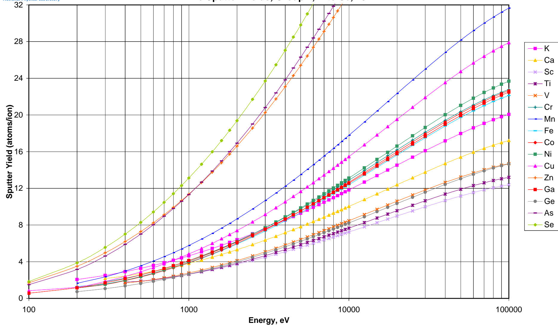
Xe Sputter Yields, Group 2, K to Se, 45°
