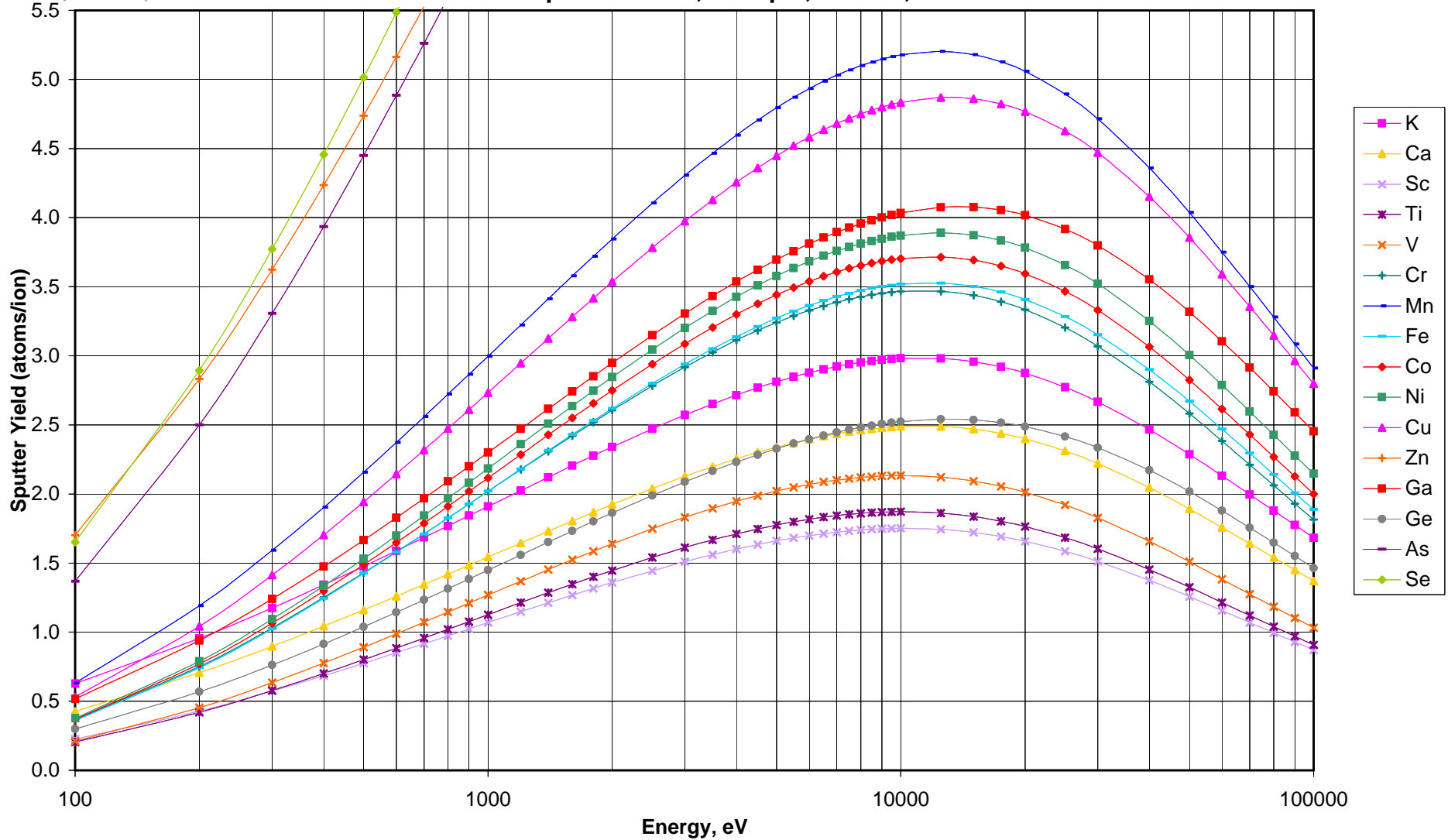
Ne Sputter Yields, Group 2, K to Se, 45°
