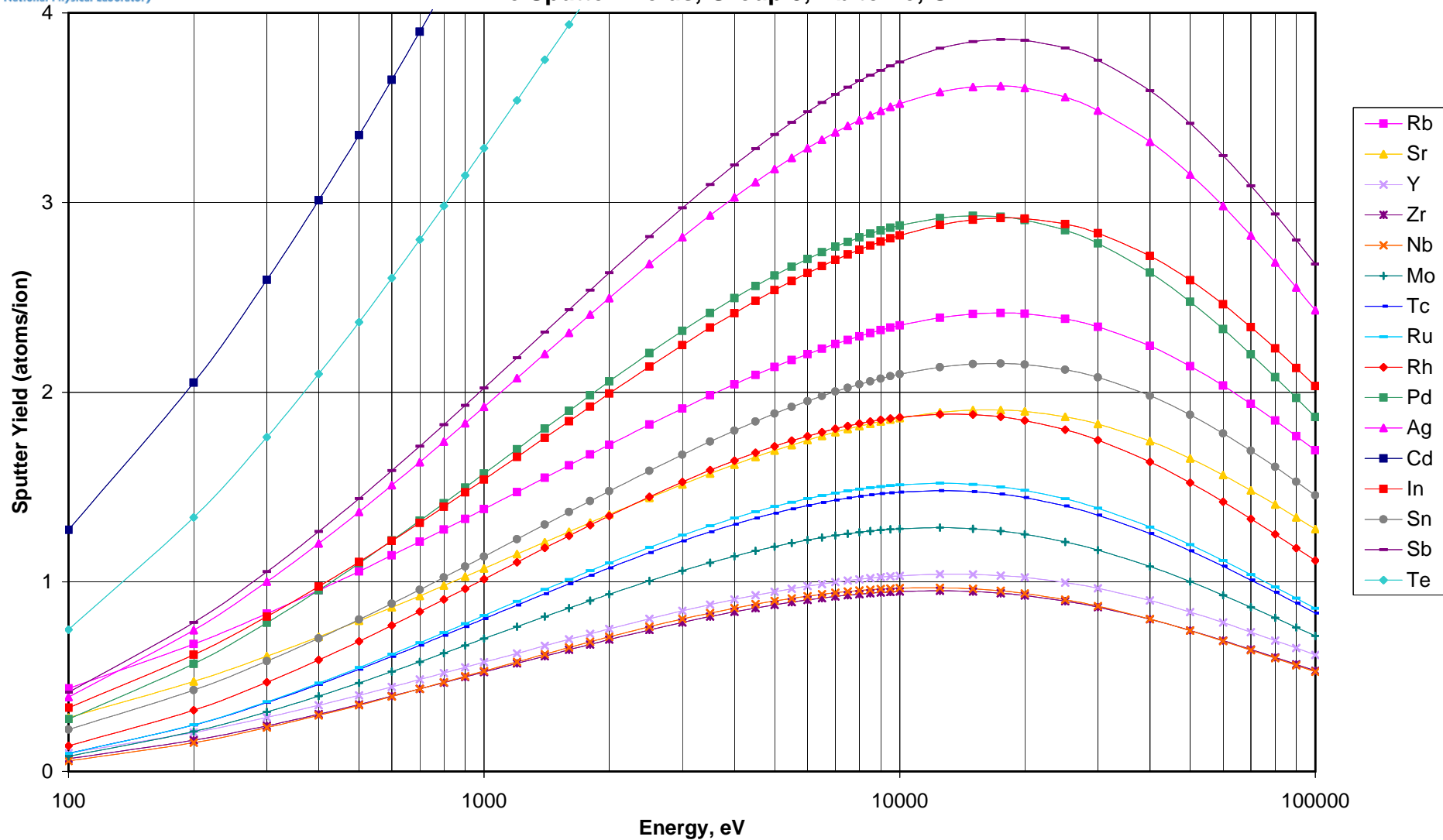
Ne Sputter Yields, Group 3, Rb to Te, 0°
