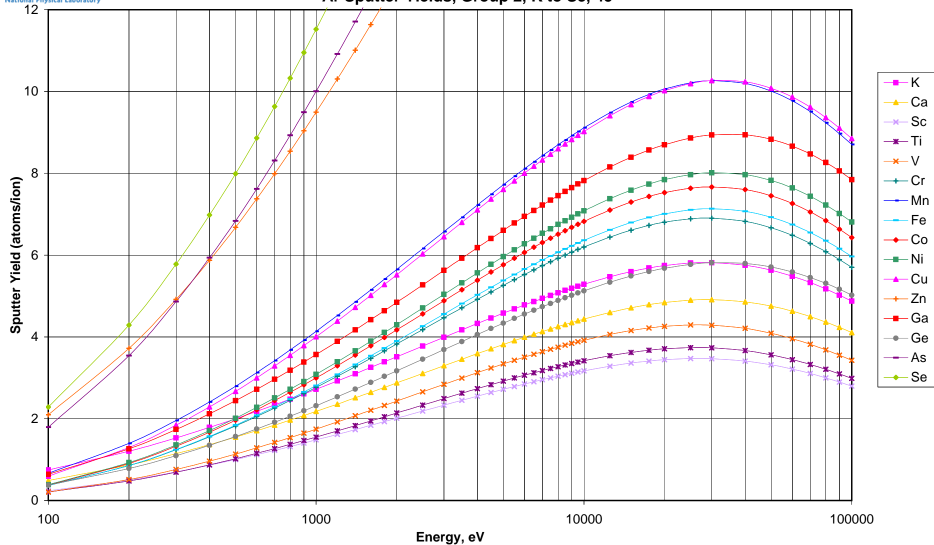
Ar Sputter Yields, Group 2, K to Se, 45°
